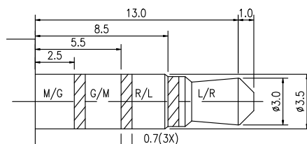
MATING PLUG
