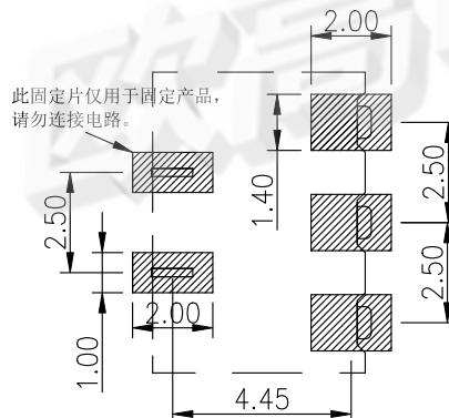
RECOMMENDED PCB LAYOUT TOP VIEW (. XX ± 0.05)
