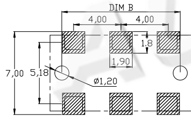
RECOMMENDED PCB LAYOUT TOP VIEW (.XX±0.05)
